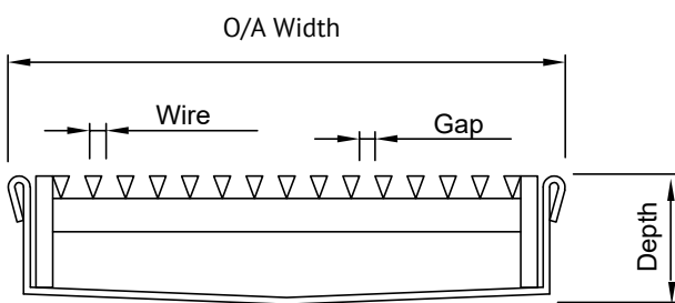
Ideal Drain with Heelguard
