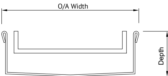
Ideal Drain with Tile Insert
